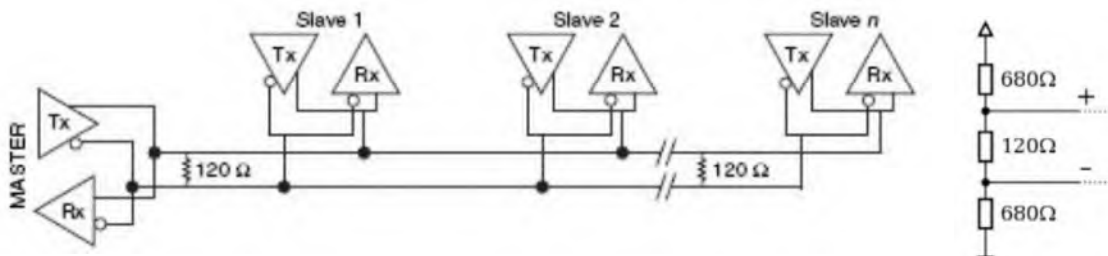
2-Wire Multidrop Network using Terminating Resistors
